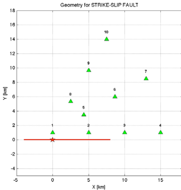
Figure 2: (Left) Source-receiver geometry for the strike-slip extended-source in map view. The red star shows the epicenter at X = 0, Y = 0 in a right-handed coordinate system with positive X pointing East, positive Y pointing North, and positive Z pointing up. The red line indicates the vertical projection of the updip-edge of an extend fault plane at depth. (Right) 3D-view of the rupture plane with an inhomogeneous slip distribution, colored-coded according to the amount of slip (in m). Small black dots indicate the x,y,z-position of kinematic rupture quantities given in the data file RuptureModel_SSEFO.dat . The black star denotes the hypocenter.
