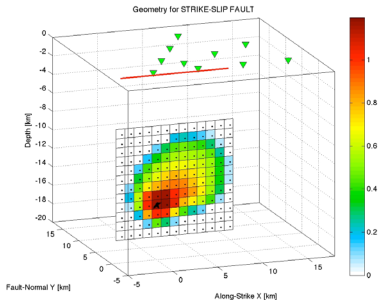
Figure 2: (Left) Source-receiver geometry for the strike-slip extended-source in map view. The red star shows the epicenter at X = 0, Y = 0 in a right-handed coordinate system with positive X pointing East, positive Y pointing North, and positive Z pointing up. The red line indicates the vertical projection of the updip-edge of an extend fault plane at depth. (Right) 3D-view of the rupture plane with an inhomogeneous slip distribution, colored-coded according to the amount of slip (in m). Small black dots indicate the x,y,z-position of kinematic rupture quantities given in the data file RuptureModel_SSEFO.dat . The black star denotes the hypocenter.
